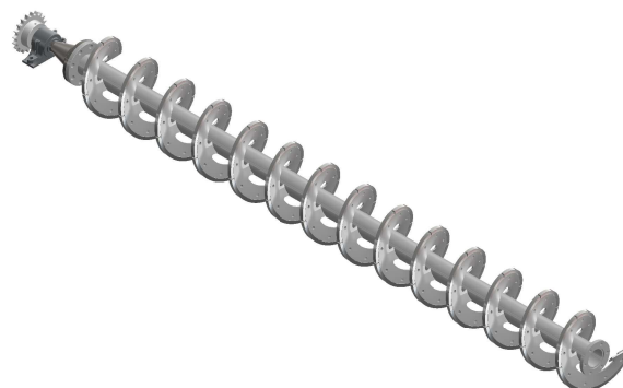
JSC 750x6500 SPIRAL CLASSIFIER SCREW PART ASSEMBLY PART NO. : JSC-300x3000-2000
