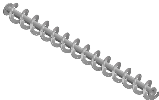
JSC 750x6500 SPIRAL CLASSIFIER MAIN SHAFT PART NO. : JSC-300x3000-2020
